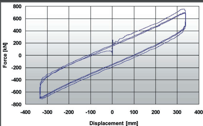
• Experimental hysteresis cycles of a double concave curved surface slider obtained in a sinusoidal test.
