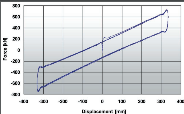
• Experimental hysteresis cycles of a double concave curved surface slider obtained in a test at constant velocity.
